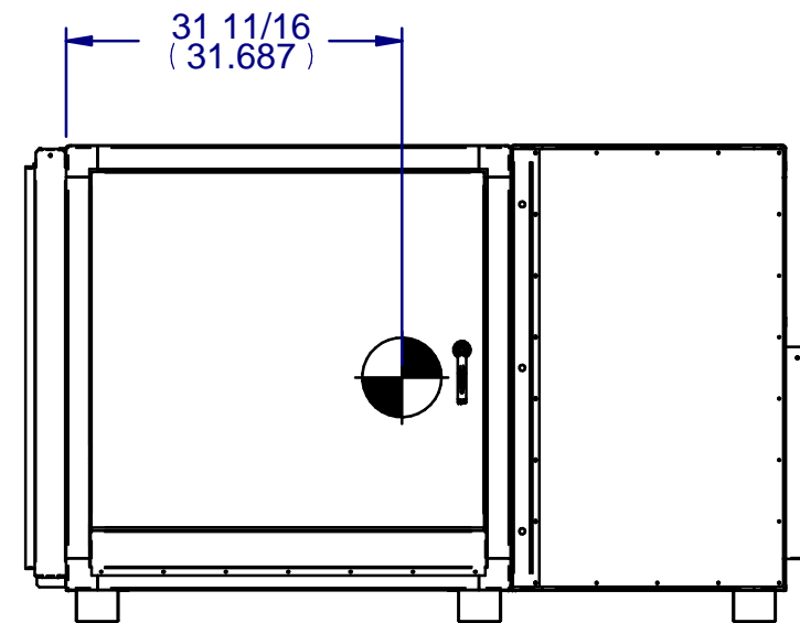
RIGHT VIEW
