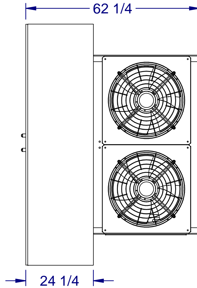
TOP VIEW
