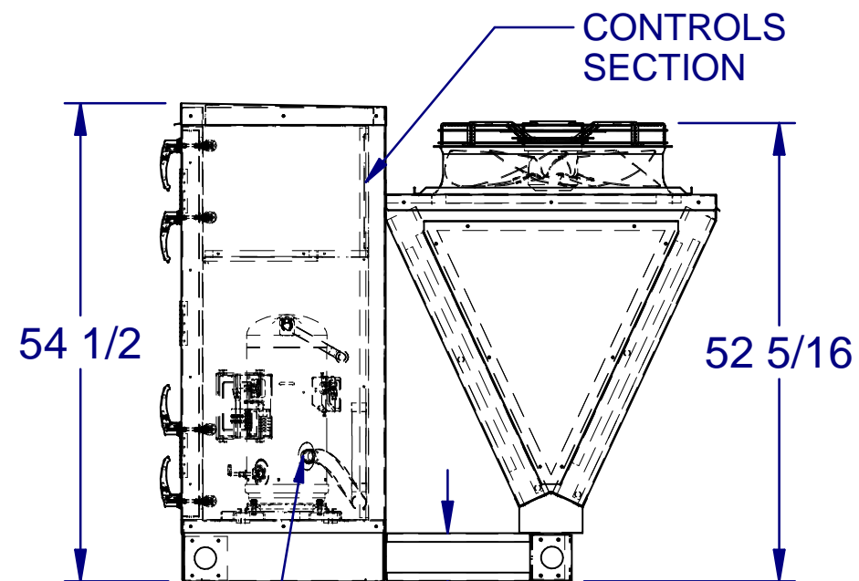
COMPRESSOR SECTION
