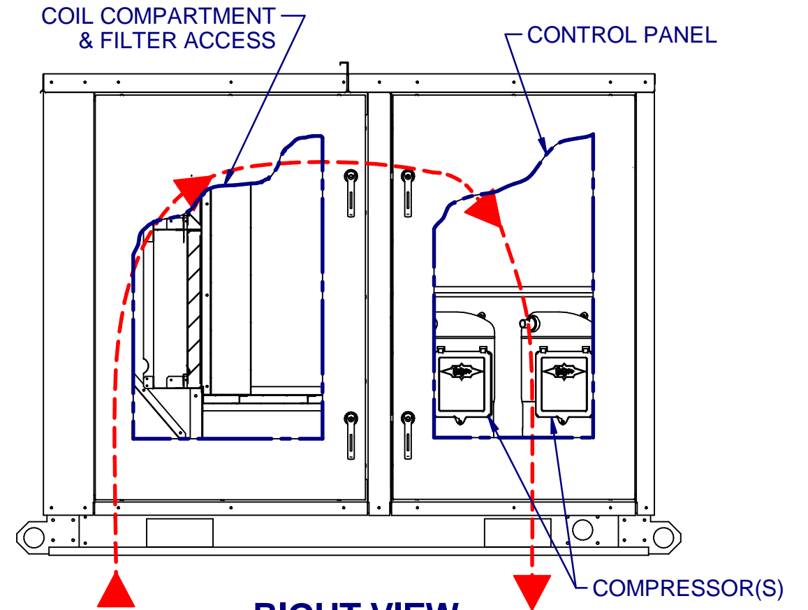
RIGHT VIEW
