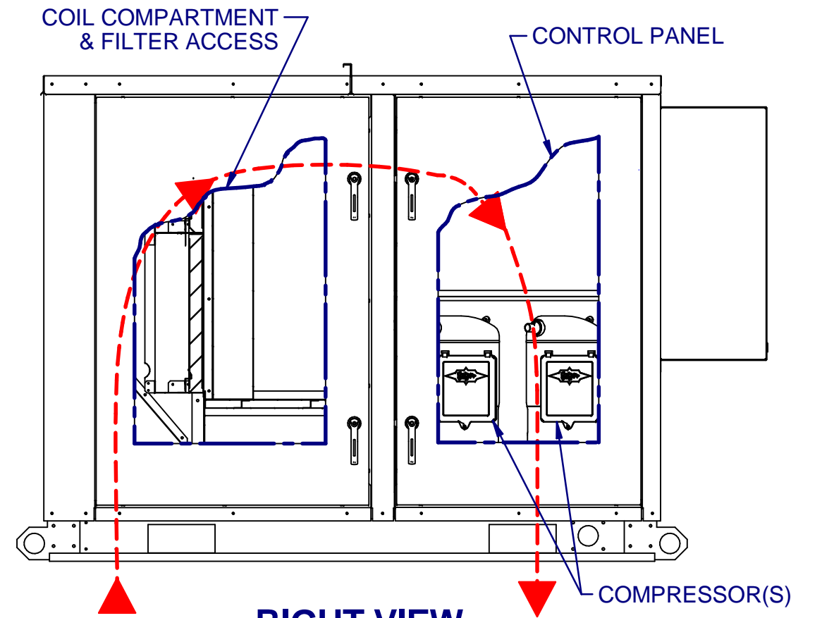
RIGHT VIEW
