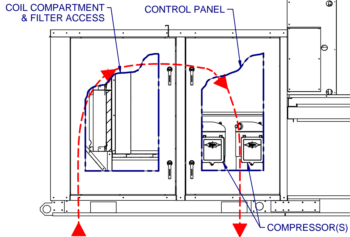
RIGHT VIEW
