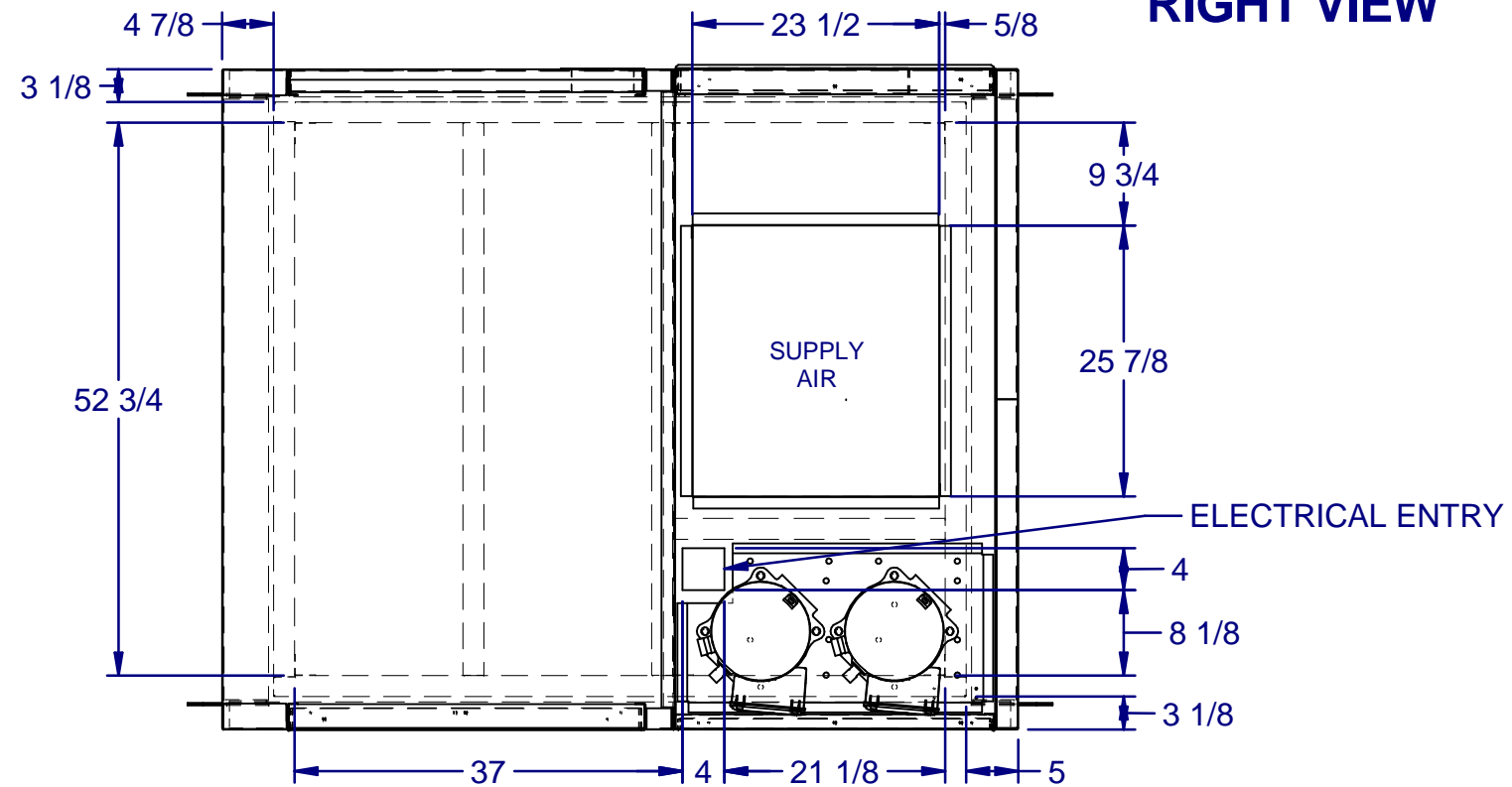
TOP PLAN VIEW CONDENSING SIDE NOT SHOWN
