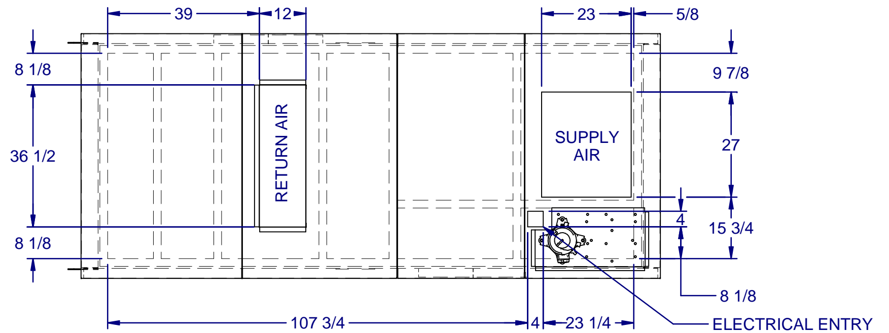
TOP PLAN VIEW CONDENSING SIDE NOT SHOWN
