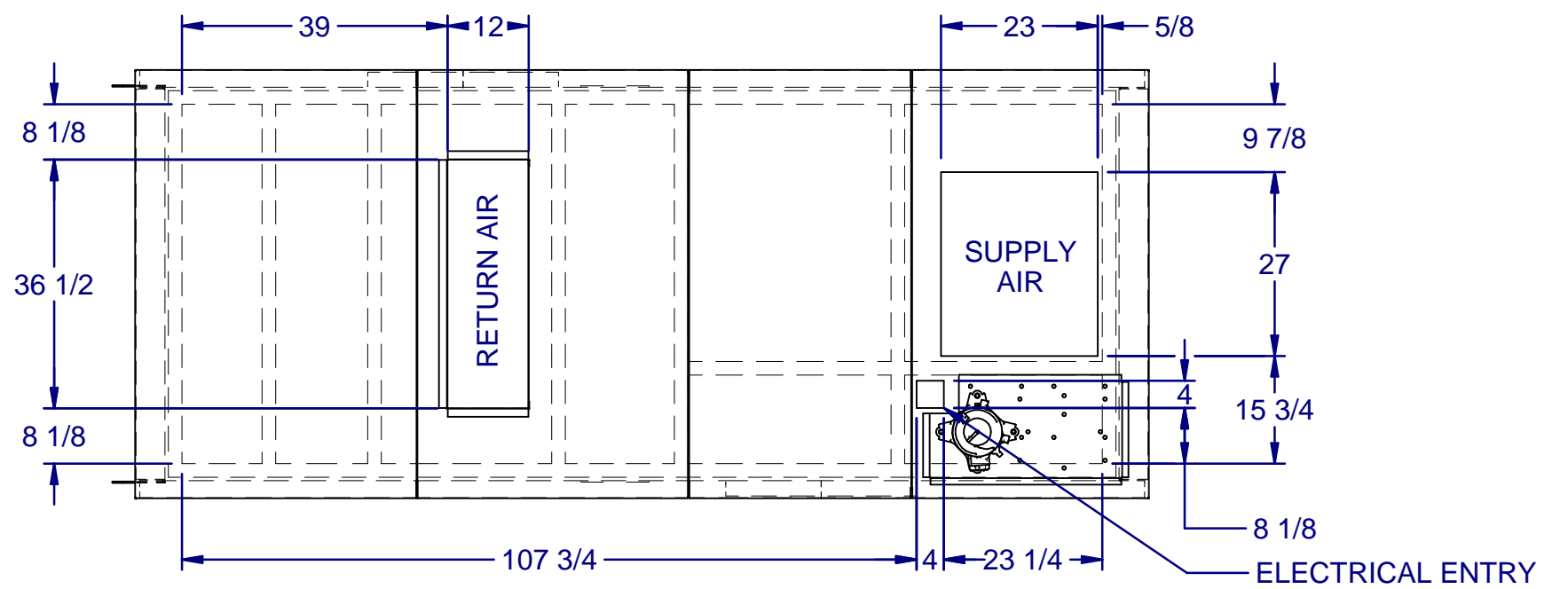
TOP PLAN VIEW CONDENSING SIDE NOT SHOWN
