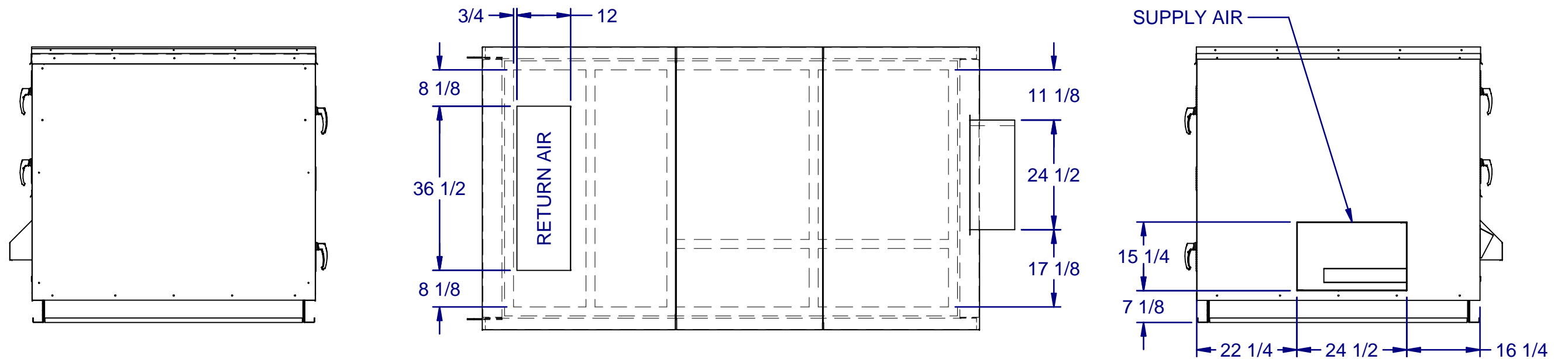
TOP PLAN VIEW CONDENSING SIDE NOT SHOWN
