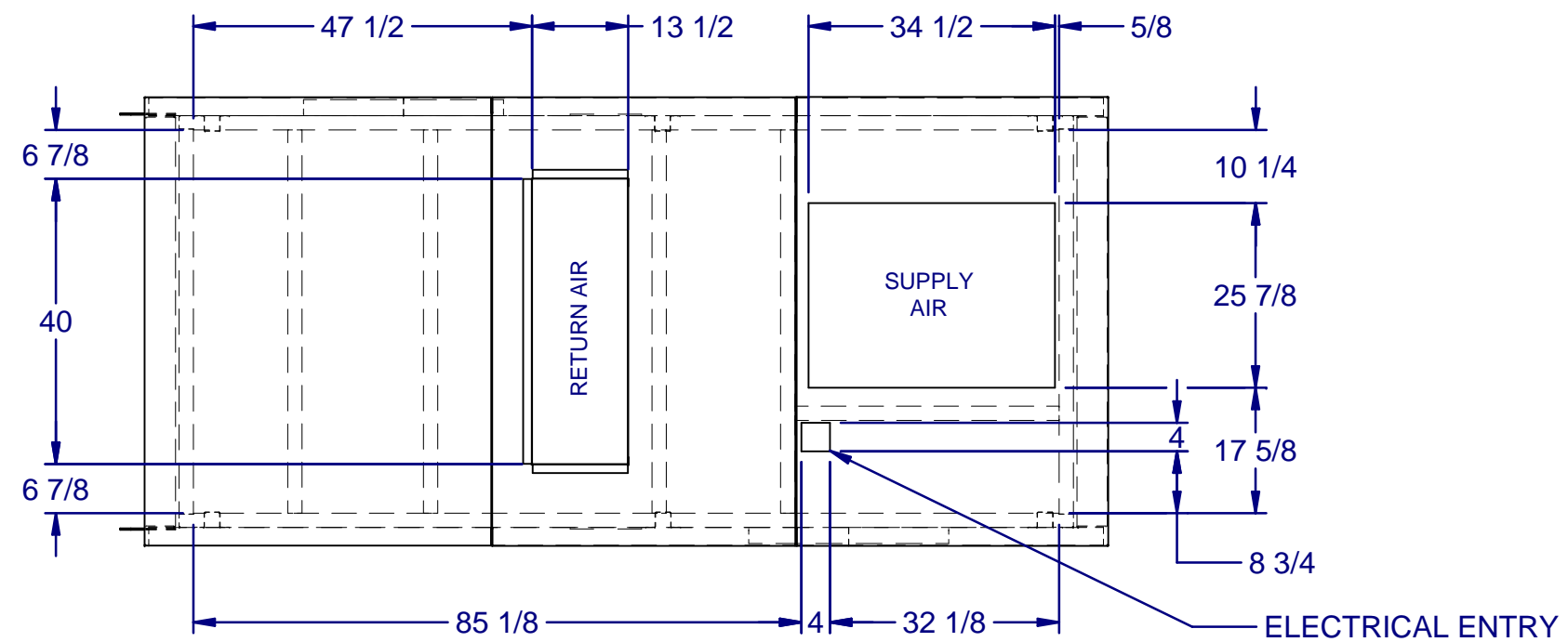
TOP PLAN VIEW CONDENSING SIDE NOT SHOWN
