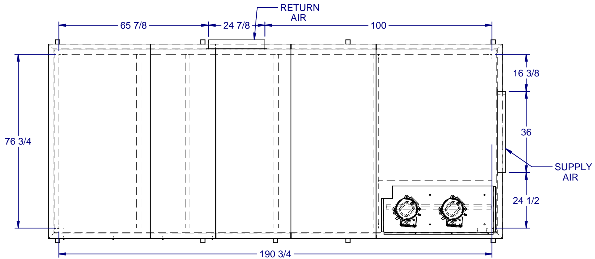
TOP PLAN VIEW CONDENSING SIDE NOT SHOWN
